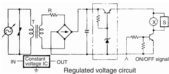
Regulated voltage circuit
