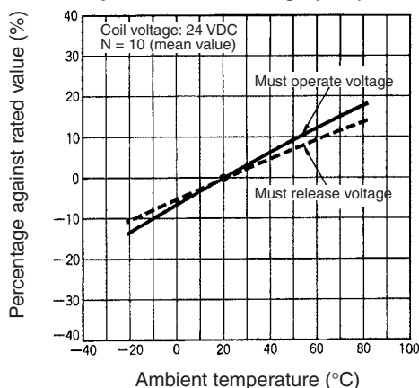
Coil Temperature vs. Must Operate/release Voltage (LZN)
